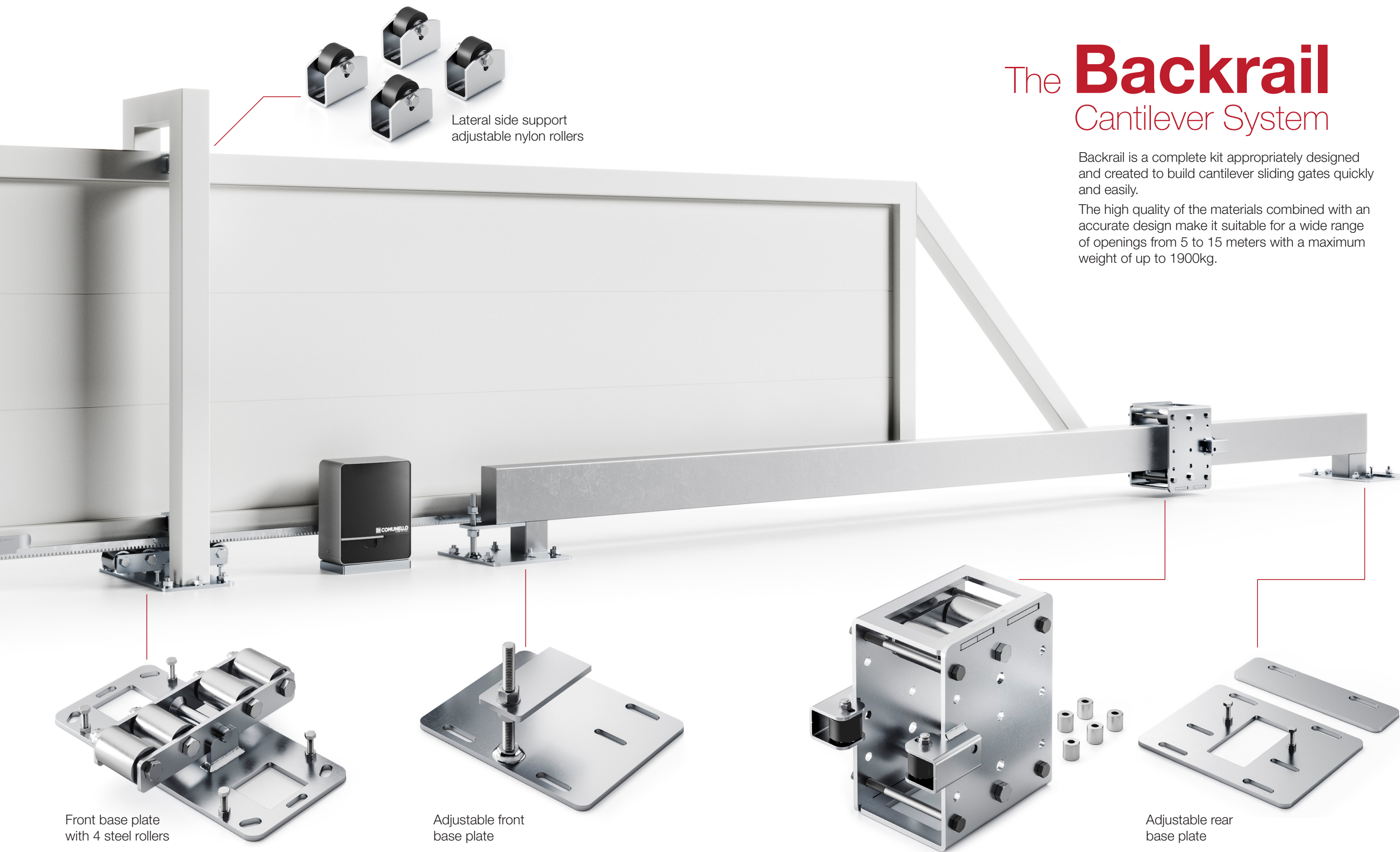
Roller box suitable for 200x100 and 150x100 backrail RHS.
